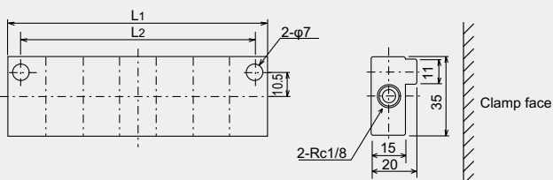
[Junction JVPA-2S]
